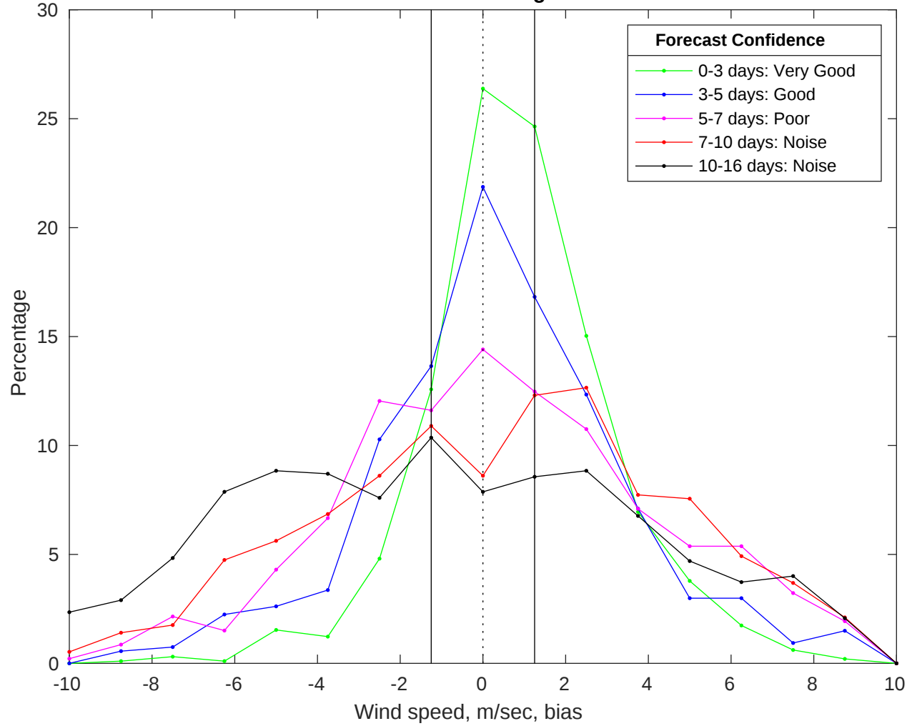
NDBC 44008 vs GFS Winds Bias Histogram: 30-Jan-2026
