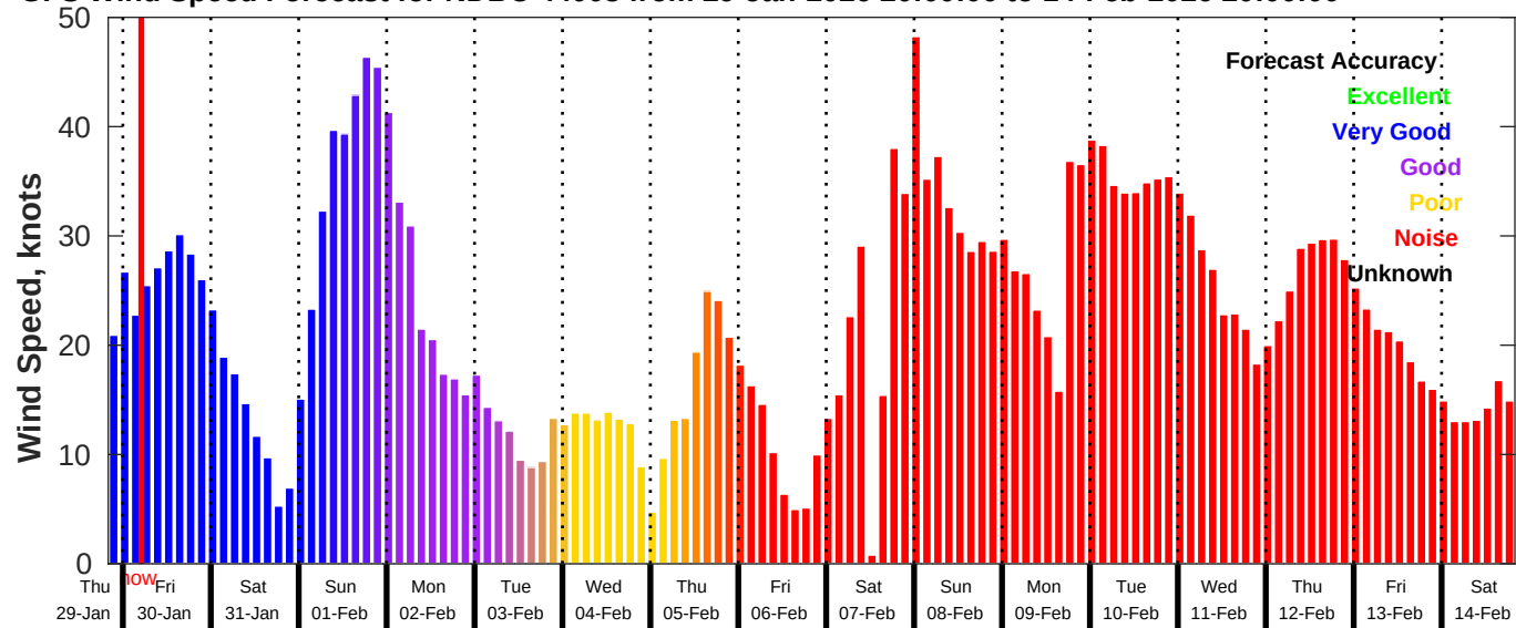
GFS Wind Speed Forecast for NDBC 44008 from 29-Jan-2026 20:00:00 to 14-Feb-2026 20:00:00
