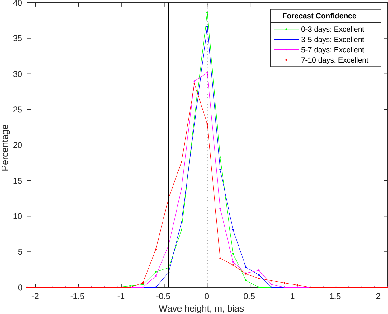
NDBC 46011 vs CMEMS Waves Bias Histogram: 30-Jan-2026
