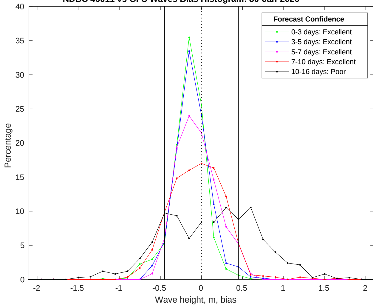
NDBC 46011 vs GFS Waves Bias Histogram: 30-Jan-2026
