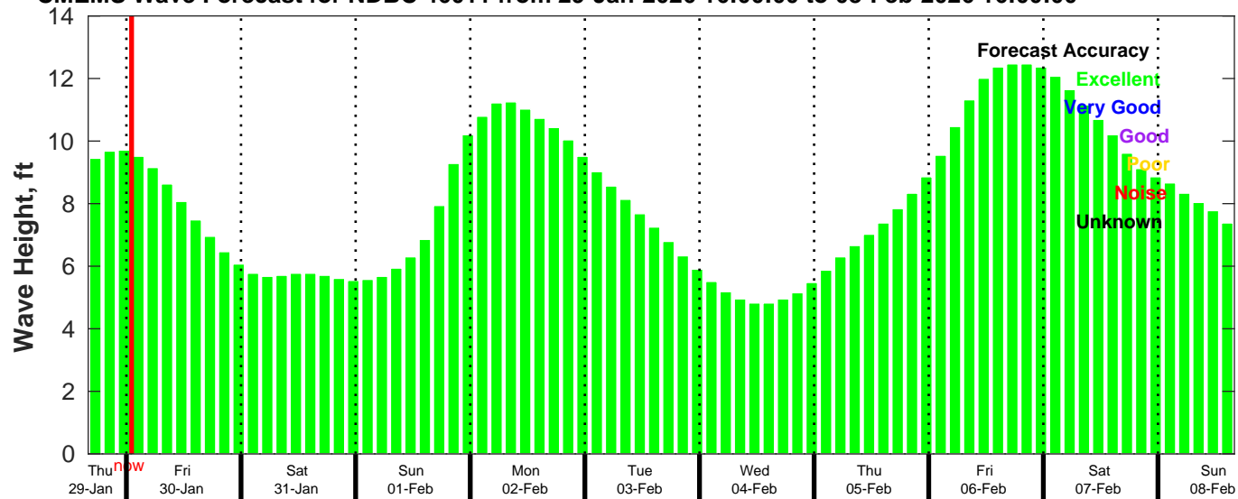
CMEMS Wave Forecast for NDBC 46011 from 29-Jan-2026 16:00:00 to 08-Feb-2026 16:00:00
