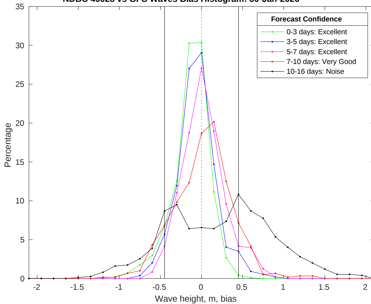
NDBC 46028 vs GFS Waves Bias Histogram: 30-Jan-2026
