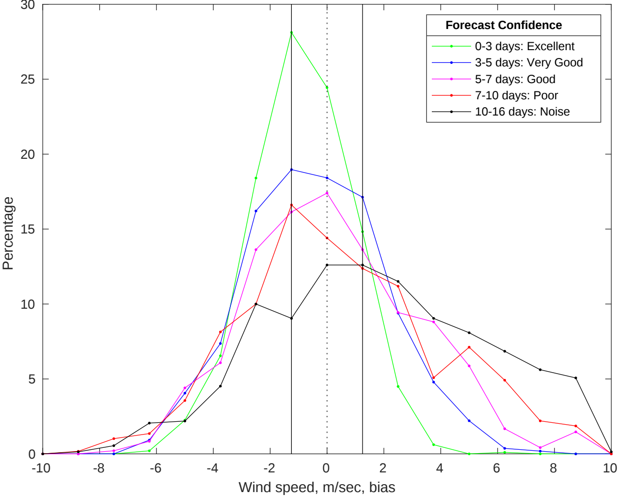
NDBC 46028 vs GFS Winds Bias Histogram: 30-Jan-2026
