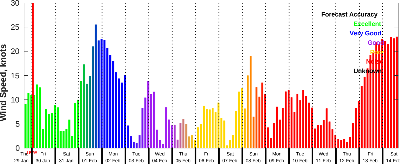
GFS Wind Speed Forecast for NDBC 46028 from 29-Jan-2026 16:00:00 to 14-Feb-2026 16:00:00
