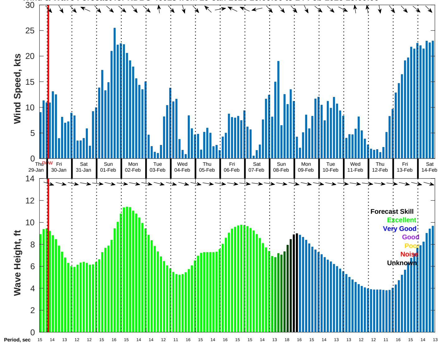
Wind & Wave Forecast for NDBC 46028 from 29-Jan-2026 16:00:00 to 14-Feb-2026 16:00:00
