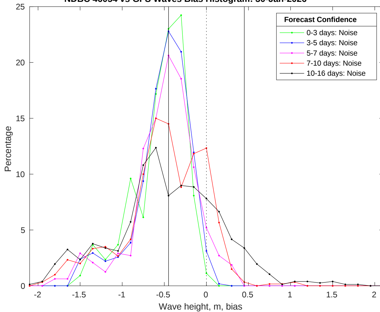
NDBC 46054 vs GFS Waves Bias Histogram: 30-Jan-2026
