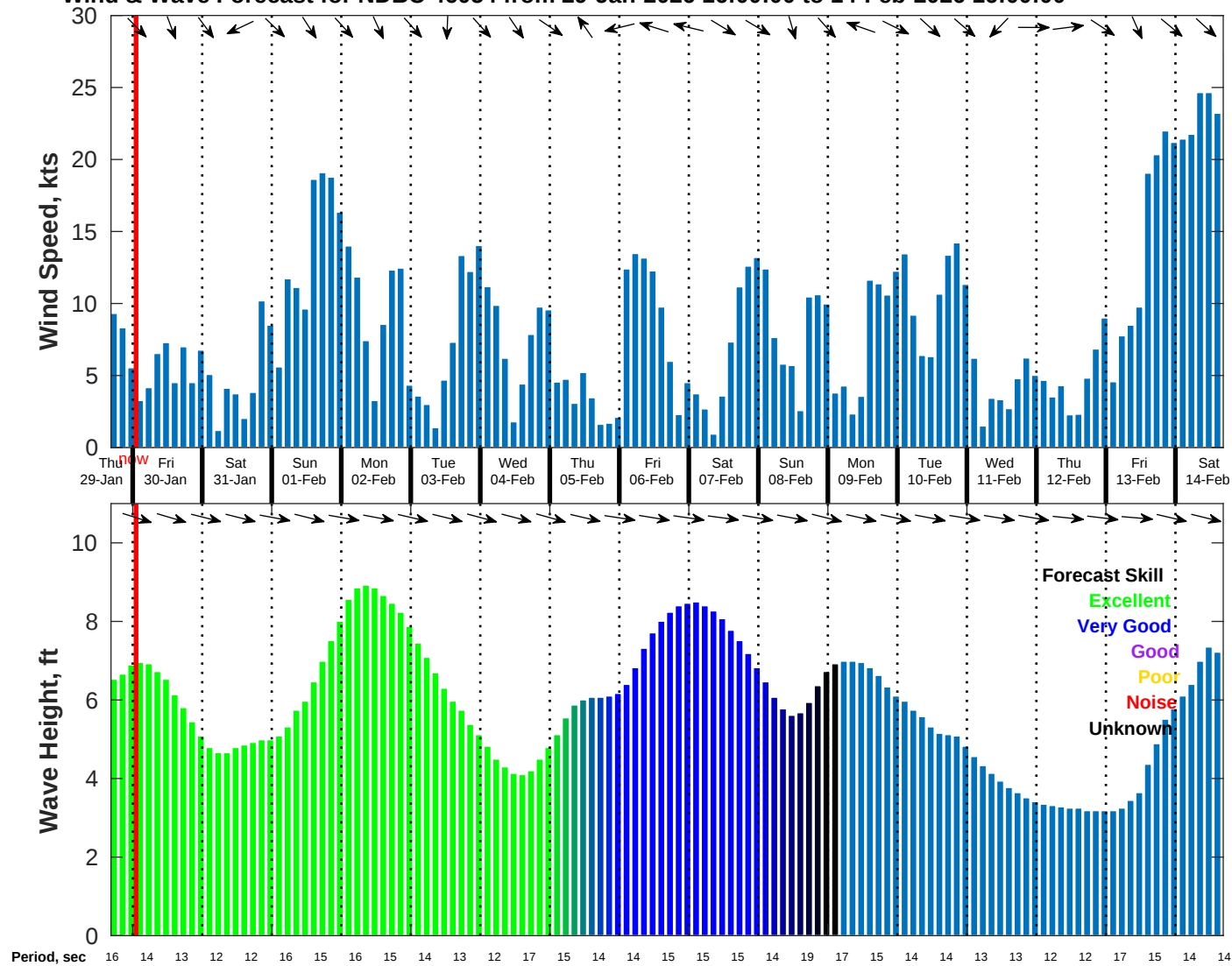
Wind & Wave Forecast for NDBC 46054 from 29-Jan-2026 16:00:00 to 14-Feb-2026 16:00:00
