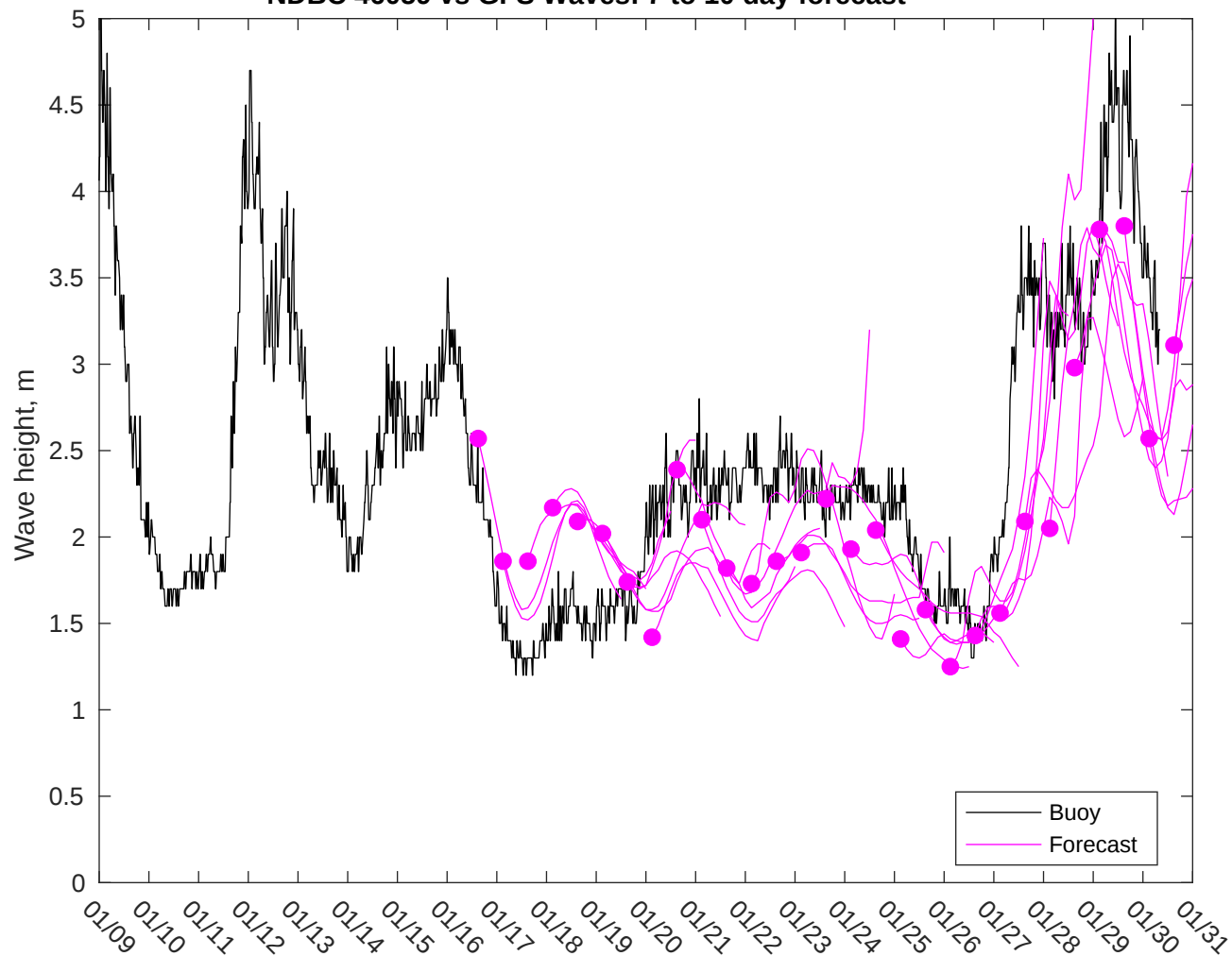
NDBC 46059 vs GFS Waves: 7 to 10 day forecast
