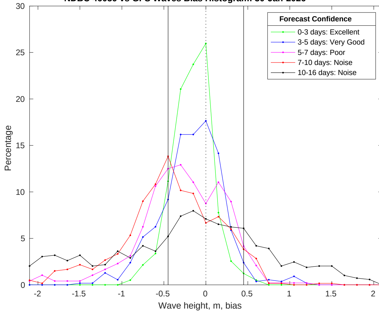
NDBC 46059 vs GFS Waves Bias Histogram: 30-Jan-2026
