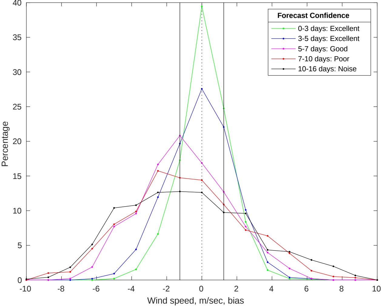
NDBC 46059 vs GFS Winds Bias Histogram: 30-Jan-2026
