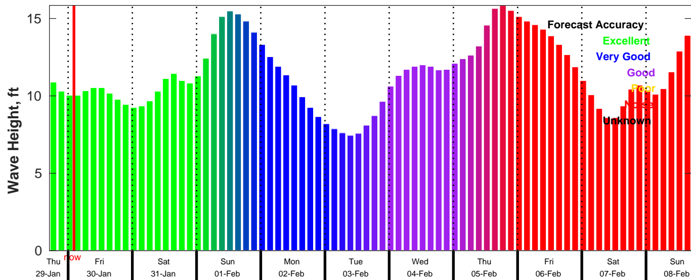
CMEMS Wave Forecast for NDBC 46059 from 29-Jan-2026 17:00:00 to 08-Feb-2026 17:00:00
