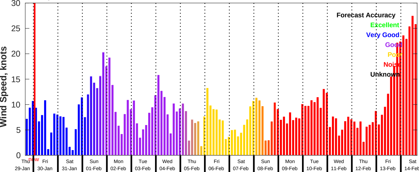
GFS Wind Speed Forecast for NDBC 46069 from 29-Jan-2026 16:00:00 to 14-Feb-2026 16:00:00
