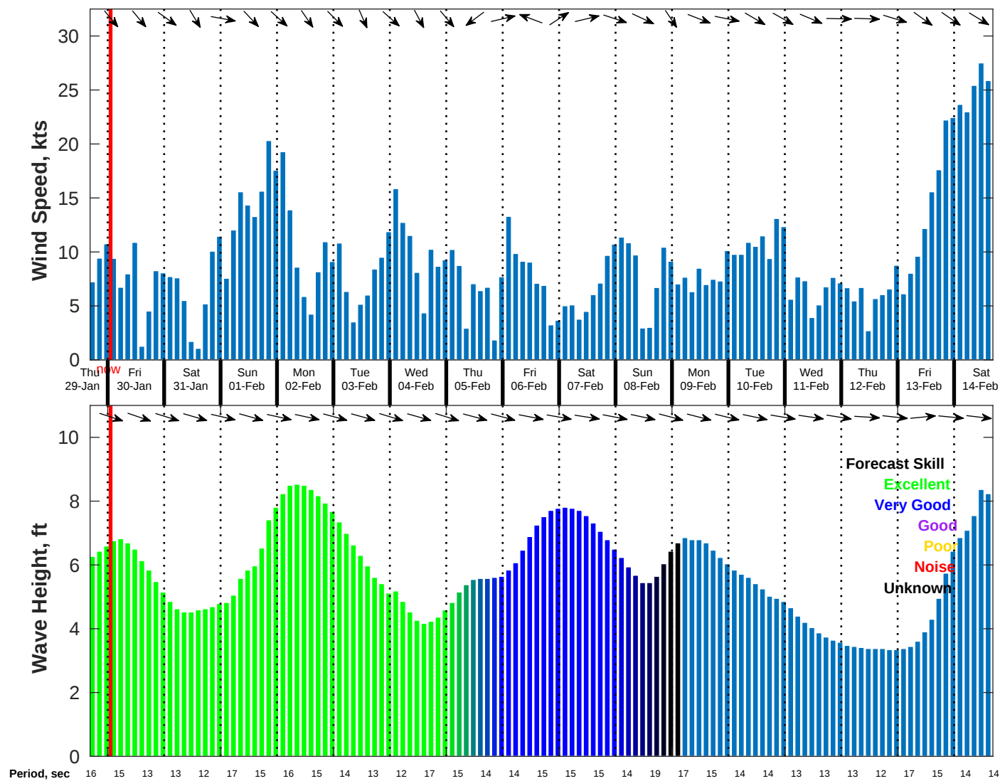
Wind & Wave Forecast for NDBC 46069 from 29-Jan-2026 16:00:00 to 14-Feb-2026 16:00:00
