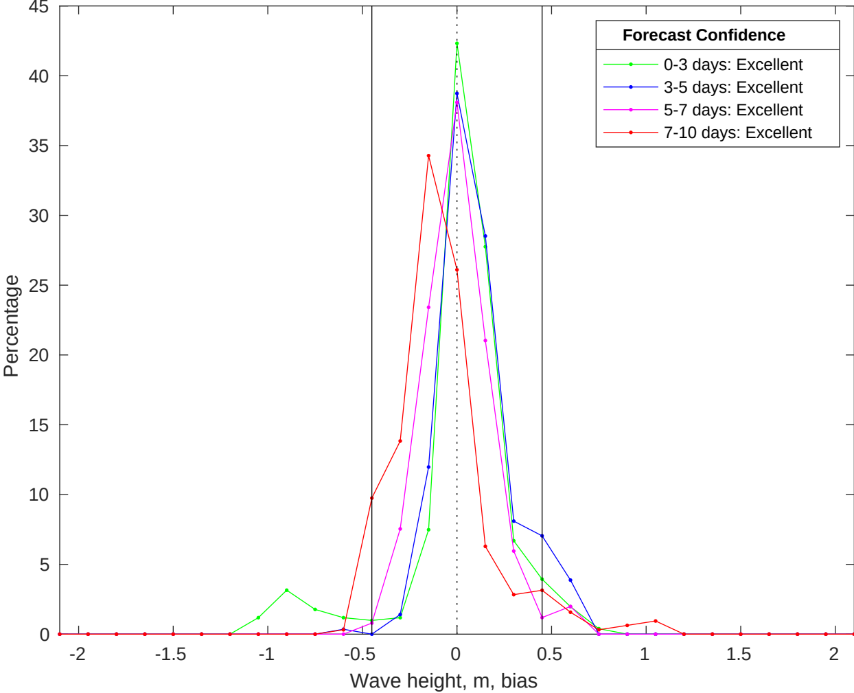
NDBC 46215 vs CMEMS Waves Bias Histogram: 30-Jan-2026
