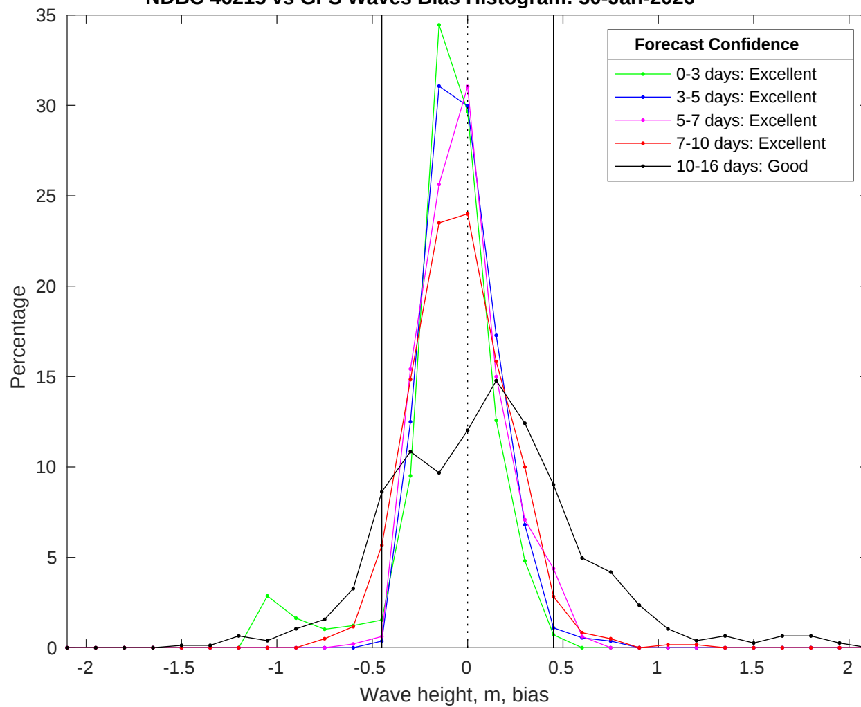
NDBC 46215 vs GFS Waves Bias Histogram: 30-Jan-2026
