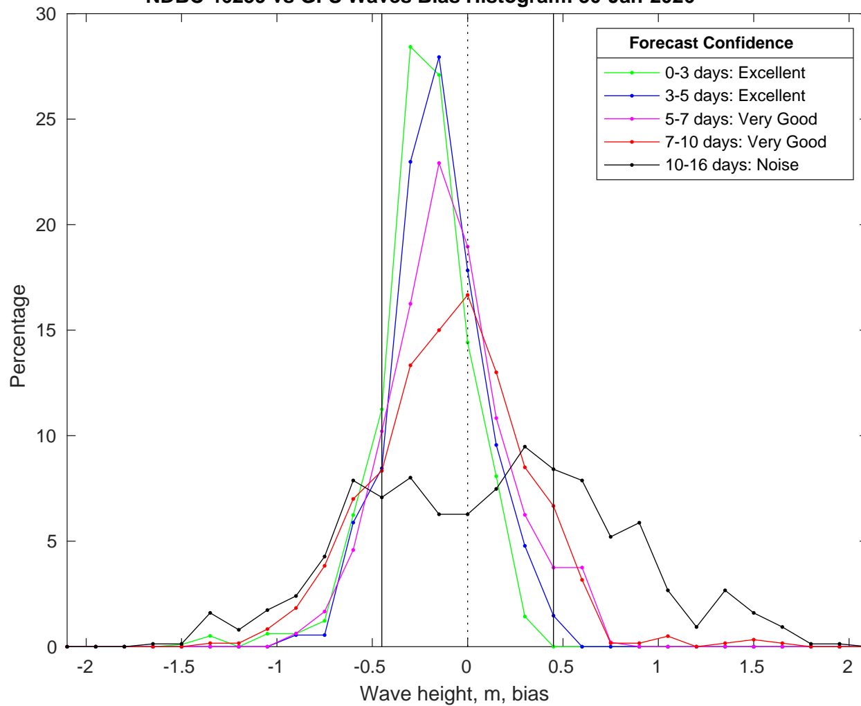
NDBC 46259 vs GFS Waves Bias Histogram: 30-Jan-2026
