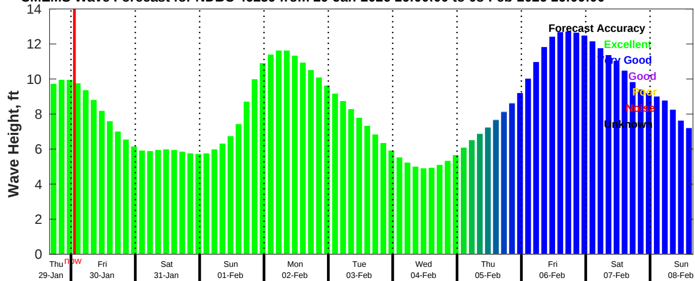
CMEMS Wave Forecast for NDBC 46259 from 29-Jan-2026 16:00:00 to 08-Feb-2026 16:00:00
