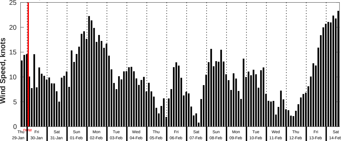
GFS Wind Speed Forecast for NDBC 46259 from 29-Jan-2026 16:00:00 to 14-Feb-2026 16:00:00
