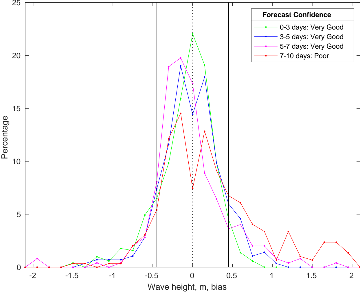
NDBC 51000 vs CMEMS Waves Bias Histogram: 30-Jan-2026
