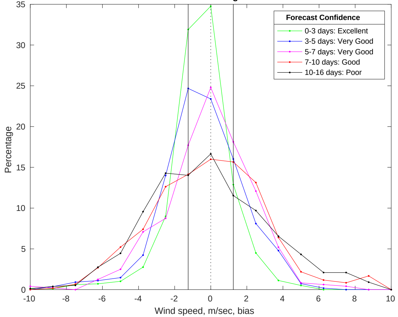
NDBC 51000 vs GFS Winds Bias Histogram: 30-Jan-2026
