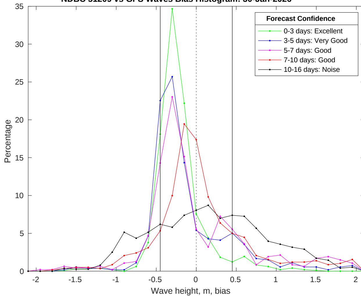
NDBC 51209 vs GFS Waves Bias Histogram: 30-Jan-2026
