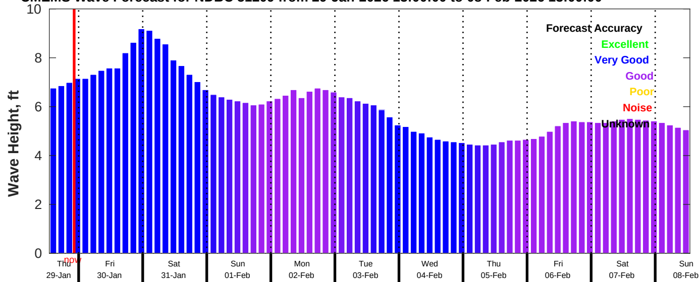
CMEMS Wave Forecast for NDBC 51209 from 29-Jan-2026 13:00:00 to 08-Feb-2026 13:00:00
