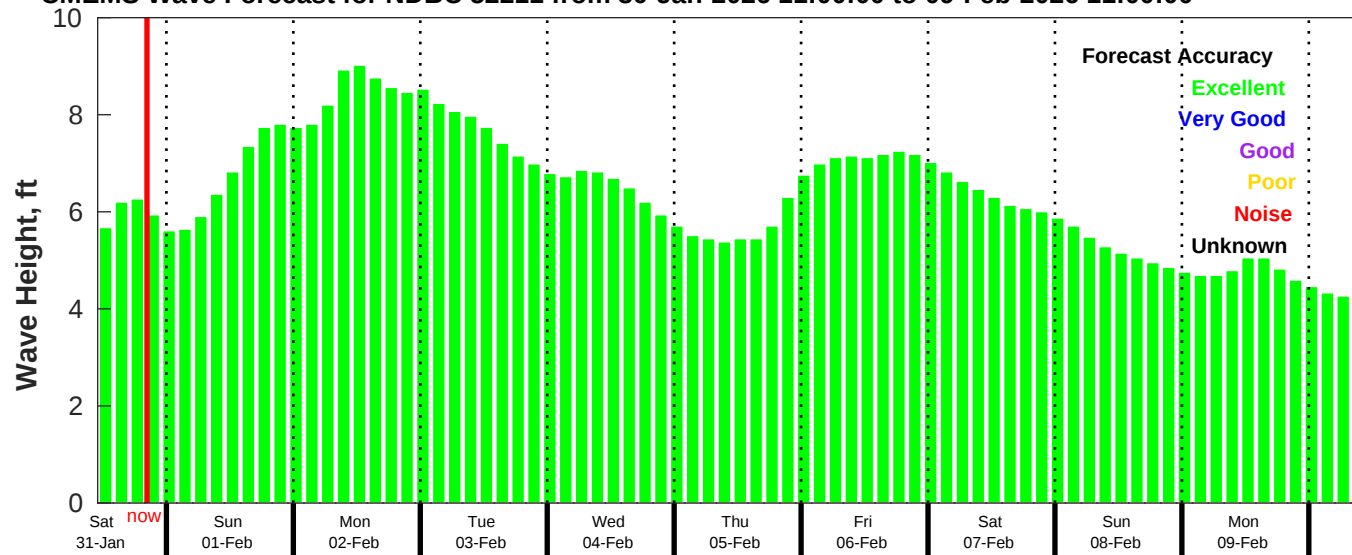
CMEMS Wave Forecast for NDBC 52211 from 30-Jan-2026 11:00:00 to 09-Feb-2026 11:00:00
