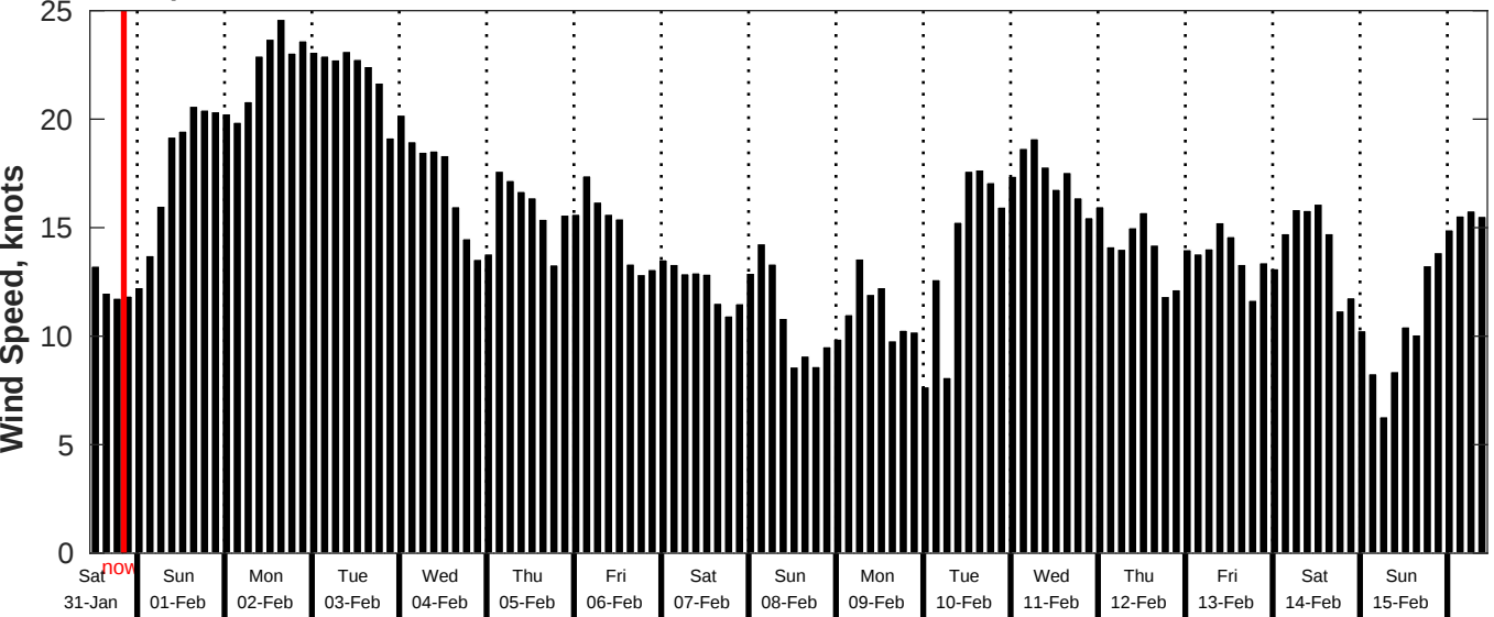
GFS Wind Speed Forecast for NDBC 52211 from 30-Jan-2026 11:00:00 to 15-Feb-2026 11:00:00
