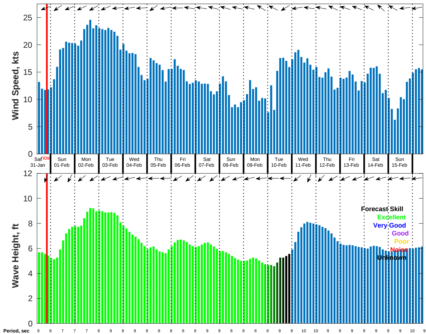
Wind & Wave Forecast for NDBC 52211 from 30-Jan-2026 11:00:00 to 15-Feb-2026 11:00:00
