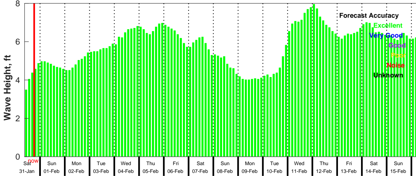
GFS Wave Forecast for NDBC 52212 from 30-Jan-2026 09:00:00 to 15-Feb-2026 09:00:00
