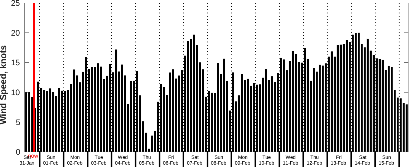
GFS Wind Speed Forecast for NDBC 52212 from 30-Jan-2026 09:00:00 to 15-Feb-2026 09:00:00
