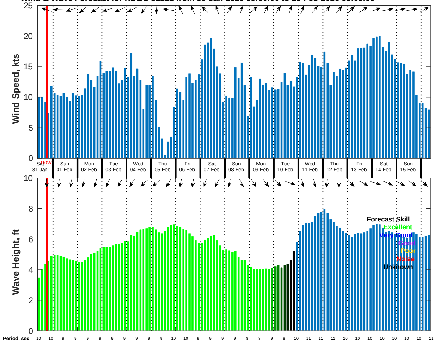
Wind & Wave Forecast for NDBC 52212 from 30-Jan-2026 09:00:00 to 15-Feb-2026 09:00:00
