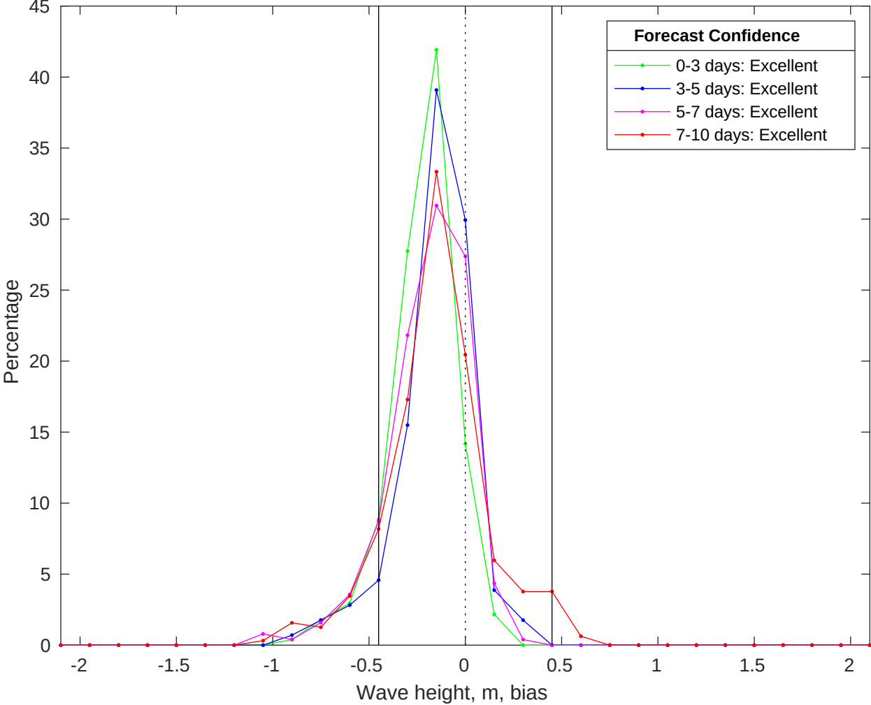
NDBC 52213 vs CMEMS Waves Bias Histogram: 30-Jan-2026
