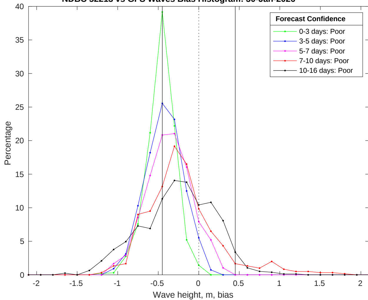
NDBC 52213 vs GFS Waves Bias Histogram: 30-Jan-2026
