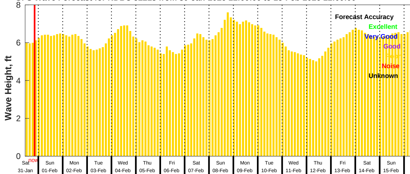
GFS Wave Forecast for NDBC 52213 from 30-Jan-2026 11:00:00 to 15-Feb-2026 11:00:00
