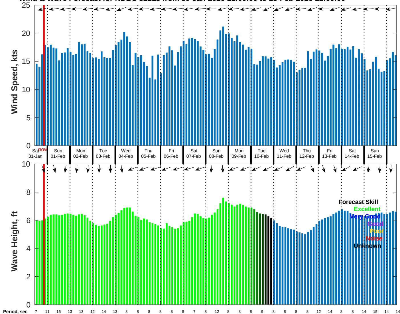
Wind & Wave Forecast for NDBC 52213 from 30-Jan-2026 11:00:00 to 15-Feb-2026 11:00:00
