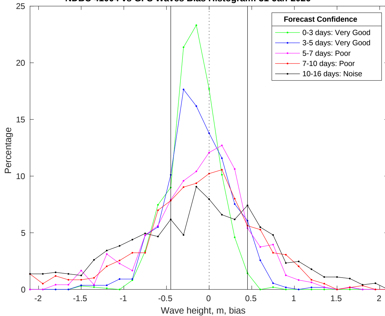
NDBC 41004 vs GFS Waves Bias Histogram: 31-Jan-2026
