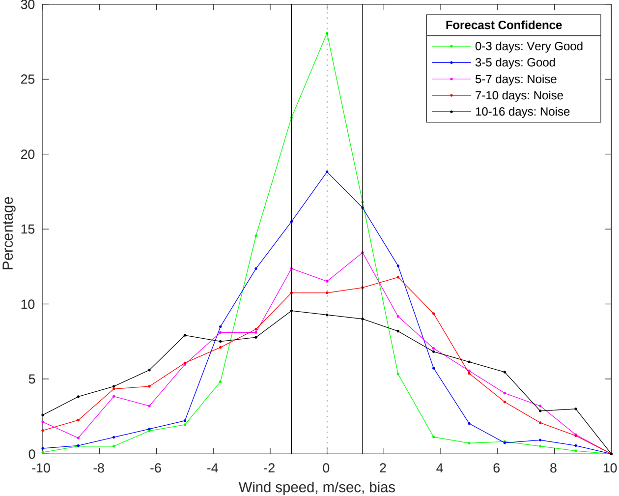
NDBC 41004 vs GFS Winds Bias Histogram: 31-Jan-2026
