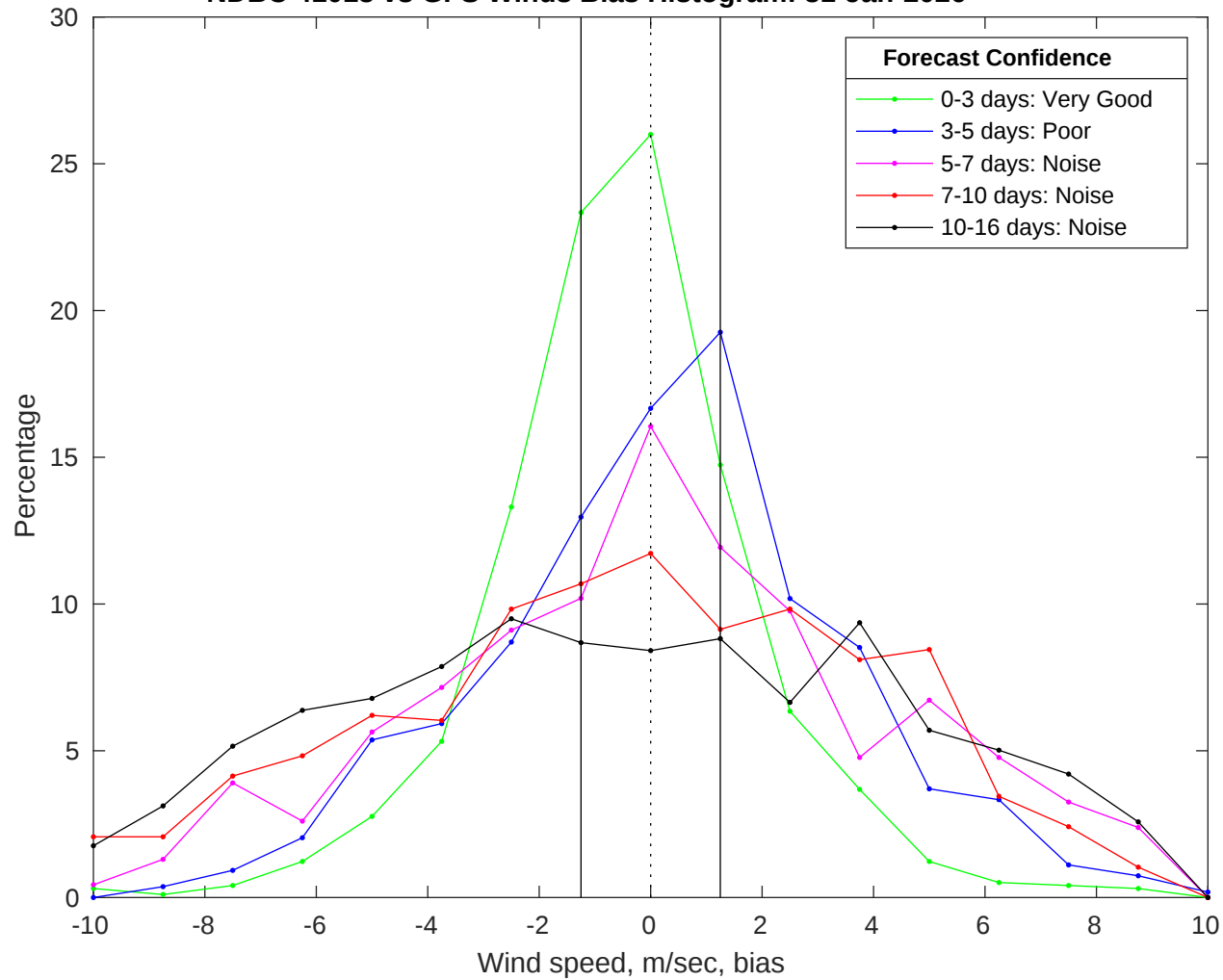
NDBC 41013 vs GFS Winds Bias Histogram: 31-Jan-2026
