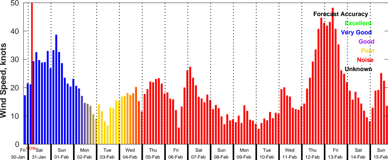
GFS Wind Speed Forecast for NDBC 41013 from 30-Jan-2026 19:00:00 to 15-Feb-2026 19:00:00
