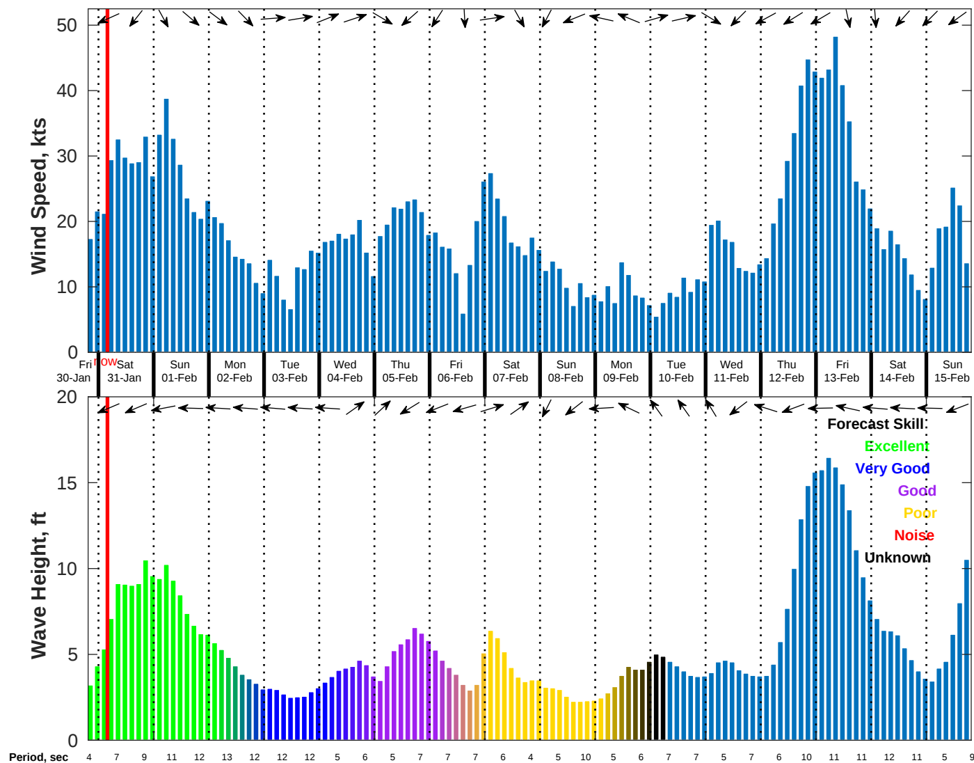
Wind & Wave Forecast for NDBC 41013 from 30-Jan-2026 19:00:00 to 15-Feb-2026 19:00:00
