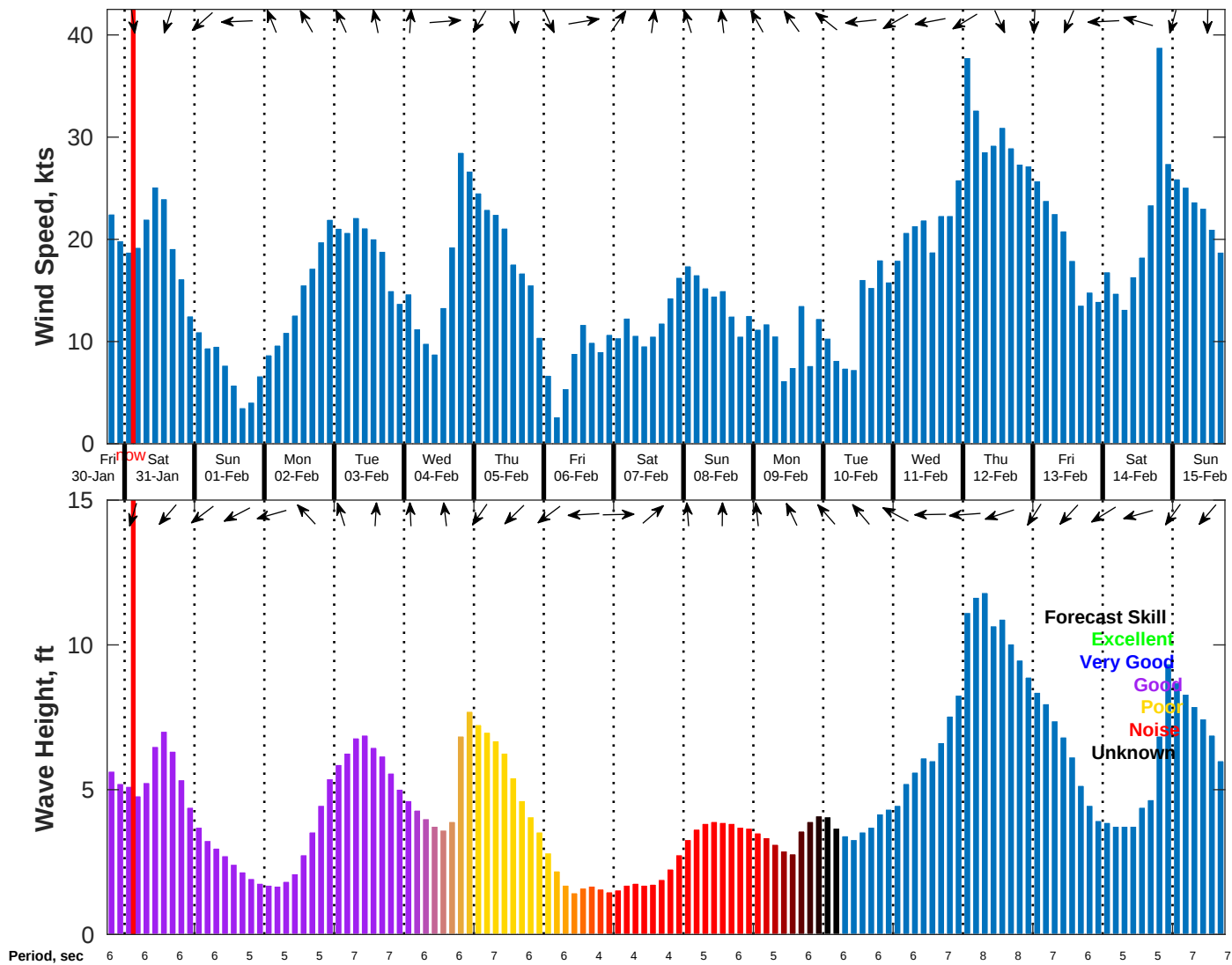
Wind & Wave Forecast for NDBC 42019 from 30-Jan-2026 18:00:00 to 15-Feb-2026 18:00:00
