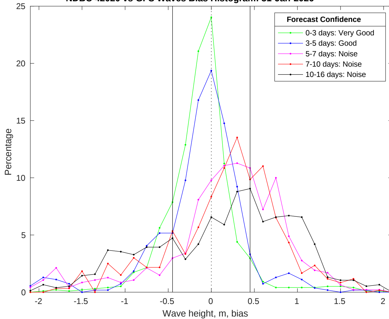
NDBC 42020 vs GFS Waves Bias Histogram: 31-Jan-2026
