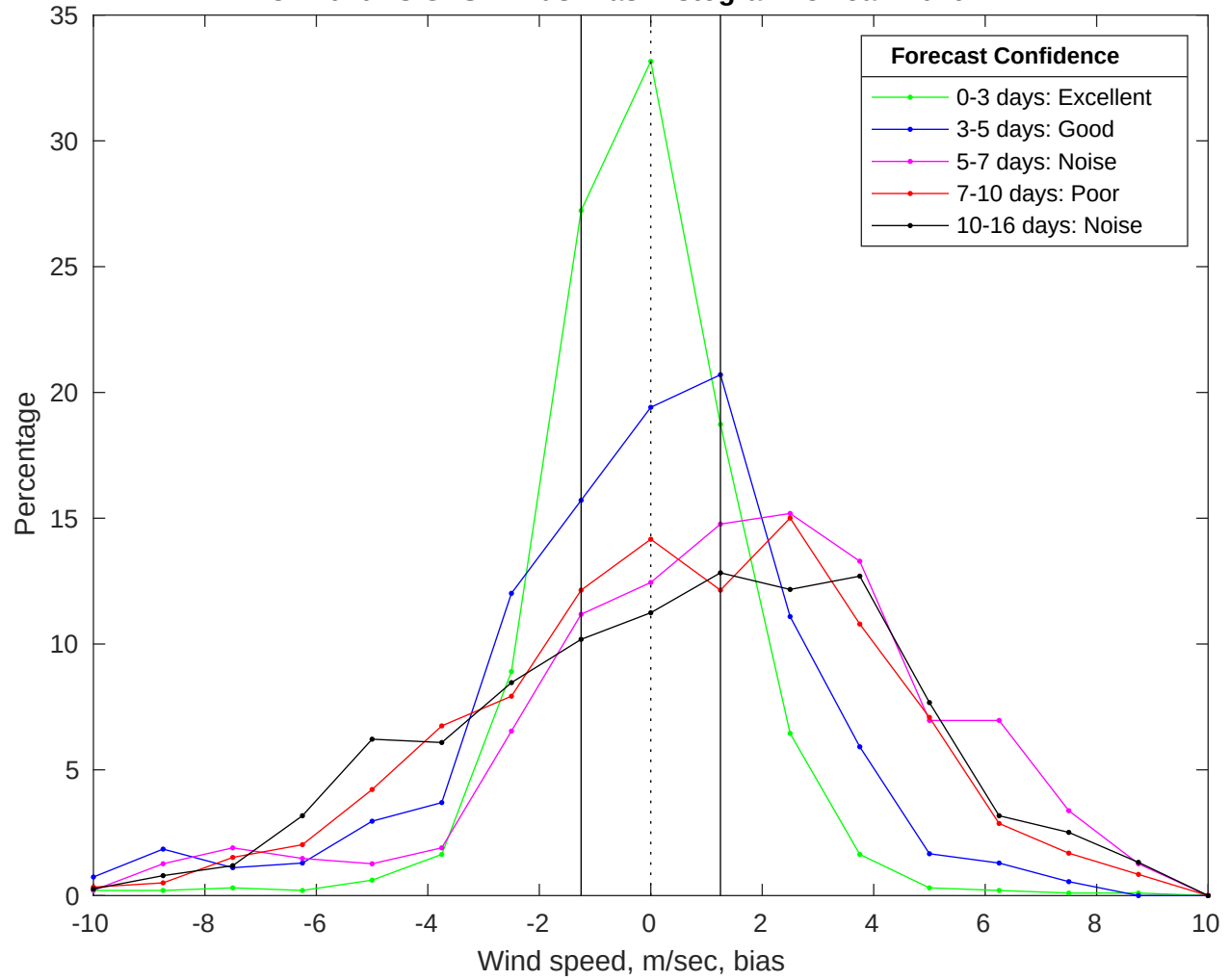
NDBC 42020 vs GFS Winds Bias Histogram: 31-Jan-2026
