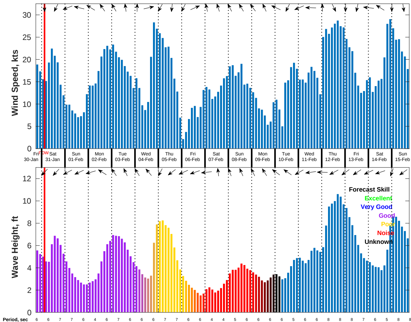
Wind & Wave Forecast for NDBC 42020 from 30-Jan-2026 18:00:00 to 15-Feb-2026 18:00:00
