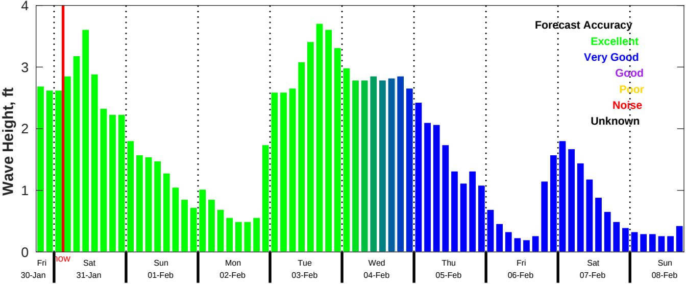
CMEMS Wave Forecast for NDBC 42035 from 30-Jan-2026 18:00:00 to 08-Feb-2026 18:00:00
