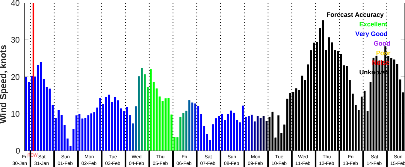
GFS Wind Speed Forecast for NDBC 42035 from 30-Jan-2026 18:00:00 to 15-Feb-2026 18:00:00
