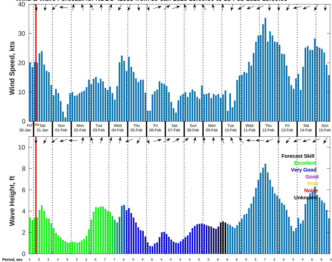
Wind & Wave Forecast for NDBC 42035 from 30-Jan-2026 18:00:00 to 15-Feb-2026 18:00:00
