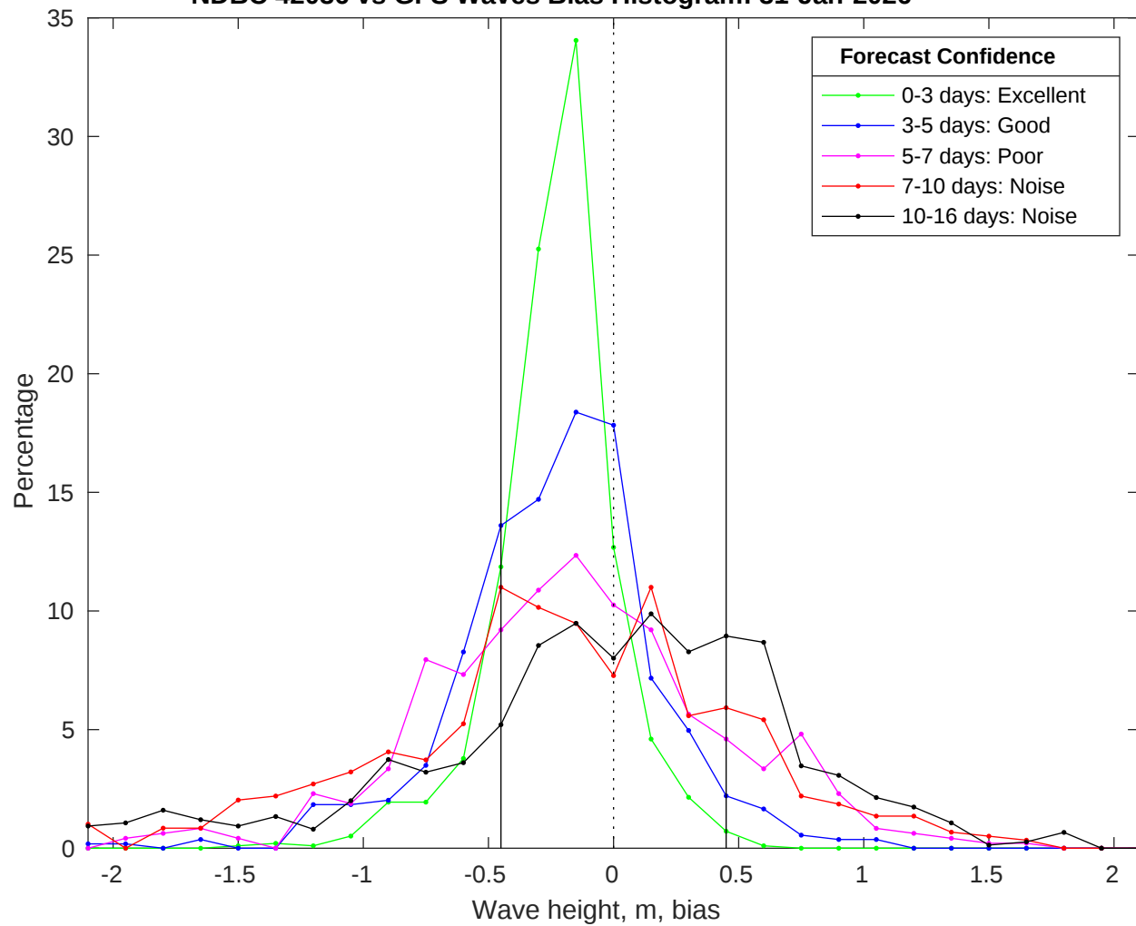
NDBC 42036 vs GFS Waves Bias Histogram: 31-Jan-2026
