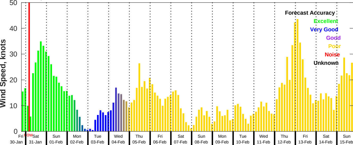
GFS Wind Speed Forecast for NDBC 42036 from 30-Jan-2026 19:00:00 to 15-Feb-2026 19:00:00
